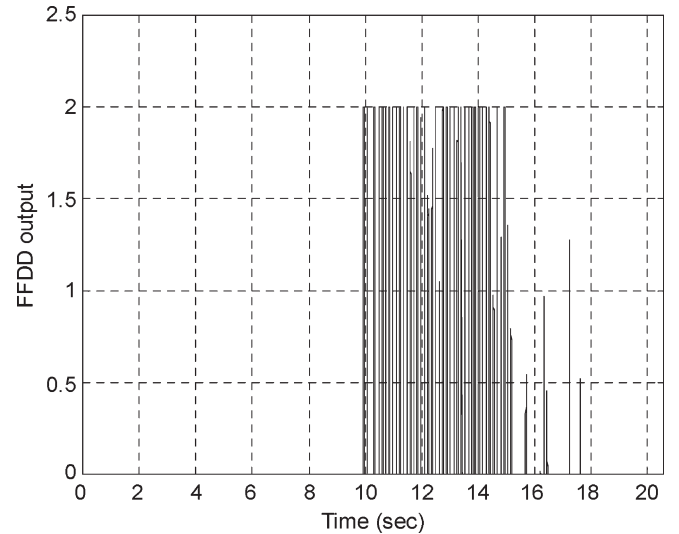
Fig. 9. FFDD output (detection of the faulty switch).
