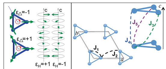
FIG. 1: from left to right: the two triangular chiralities \epsilon_{\Delta} = \pm 1 , the two helicities \epsilon_H = \pm 1 , and the magnetic exchange paths J_1 to J_5 in \text{Ba}_3\text{NbFe}_3\text{Si}_2\text{O}_{14} .
