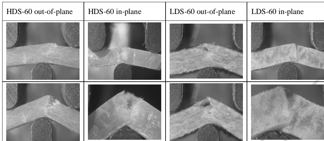
Figure 11. Sequences of in-situ micrographs during three-point bending of the 3 mm thick LDS and HDS composite samples in wet conditions after saturation in water.
