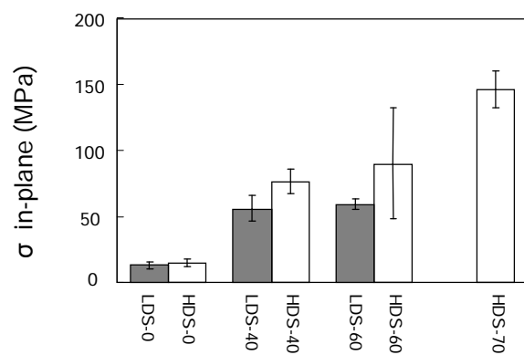
Figure 8. In-plane strength in three-point bending of thermoset starch composites. The error bars indicate standard deviations.
