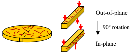
Figure 6. Test directions in three point bending of the composite disks with in-plane random fibre orientation distribution.
