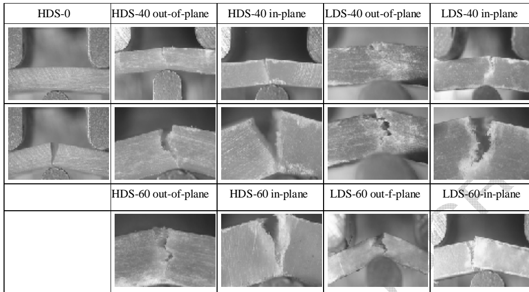
Figure 10. Sequences of in-situ micrographs during three-point bending of the 3 mm thick LDS and HDS composite samples in dry conditions.
