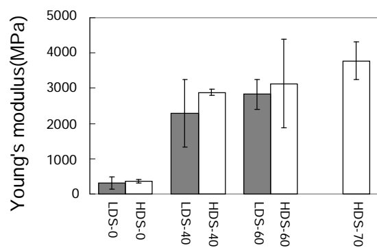
Figure 7. In-plane Young's modulus of thermoset starch composites. The error bars indicate standard deviations.
