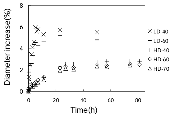
Figure 5. Diameter increase (in-plane hygroscopic strain) with immersion time in water of flat cylindrical specimens of LDS and HDS composites.
