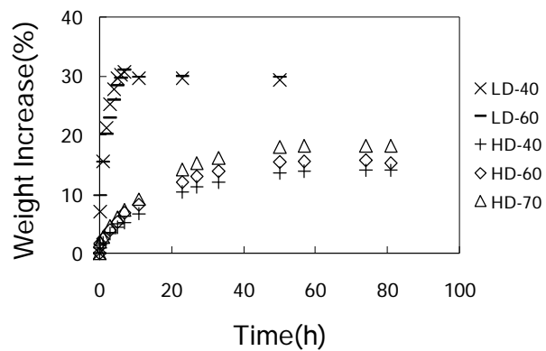
Figure 3. Weight increase of LDS and HDS composites with immersion time in water.
