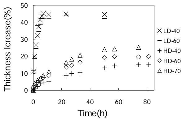
Figure 4. Thickness increase of LDS and HDS composites (out-of-plane hygroscopic strain) with immersion time in water.
