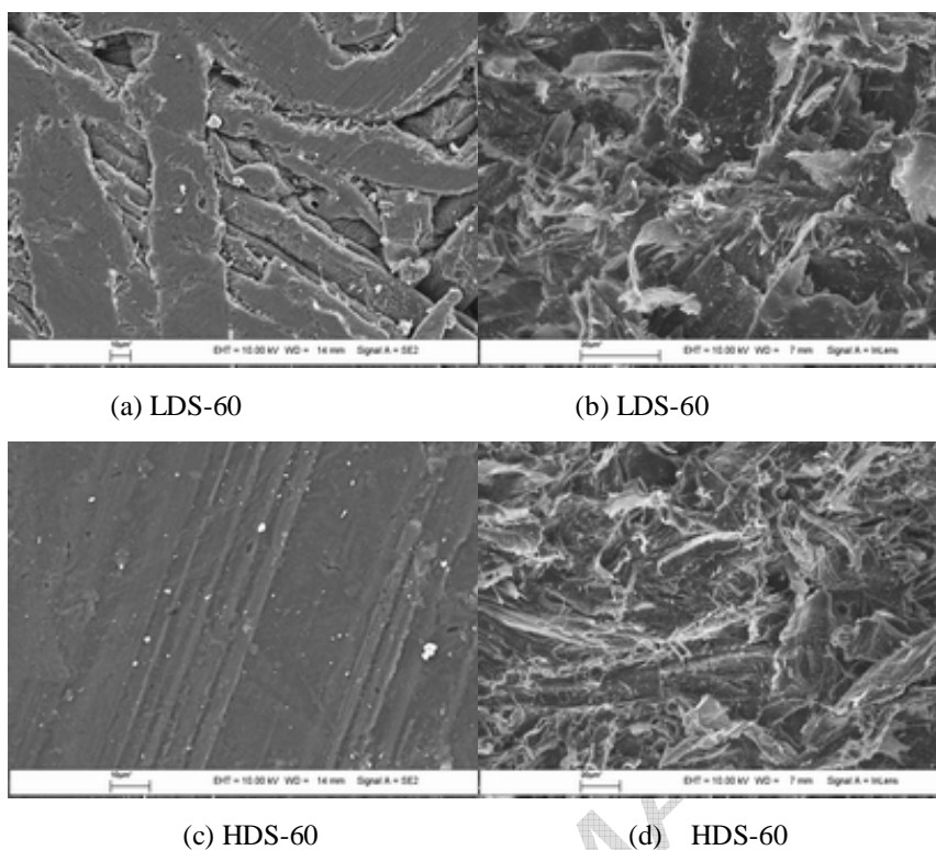
Figure.1 SEM images of LDS-60 composite at (a) the mould-face surface with 500 \times magnification, at (b) a fracture surface with 1000 \times magnification, and of HDS-60 composite at (c) the mould-face surface with 1000 \times magnification, and at (d) a fracture surface with 500 \times magnification.
