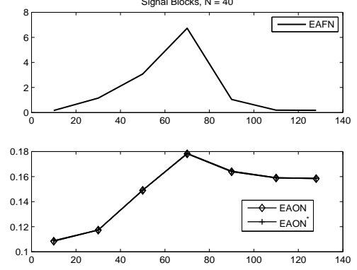
Figure 12(b). Values of EAFN , EAON and EAON^* for Signal Blocks as a function of n
