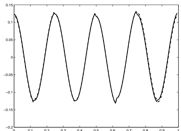
Figure 6(b). Signal F_2 and Eigenvector associated to the second largest eigenvalue of \hat{\Sigma}_f with G = [G^1 \ G^2]
