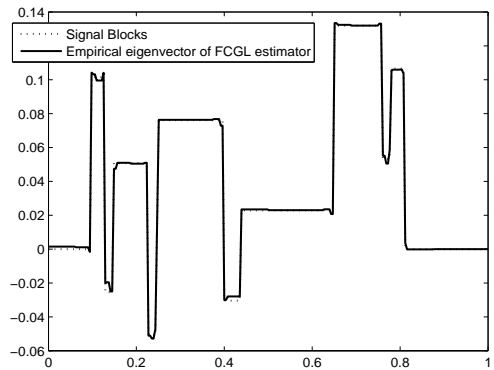
Figure 3(b). Signal Blocks and Eigenvector associated to the largest eigenvalue of \widehat{\Sigma}_{\hat{\lambda}}
