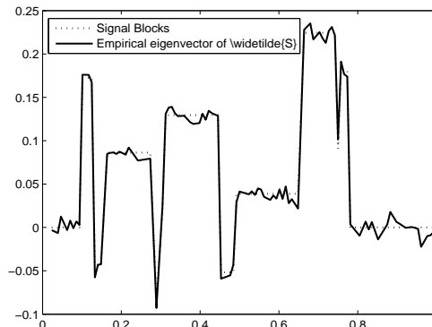
Figure 8(b). Signal Blocks and Eigenvector associated to the largest eigenvalue of \tilde{S}
