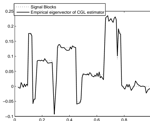
Figure 8(b). Signal Blocks and Eigenvector associated to the largest eigenvalue of \tilde{S}
