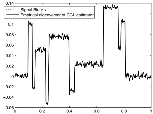
Figure 2(b). Signal Blocks and Eigenvector associated to the largest eigenvalue of \widehat{\Sigma}_{\lambda}
