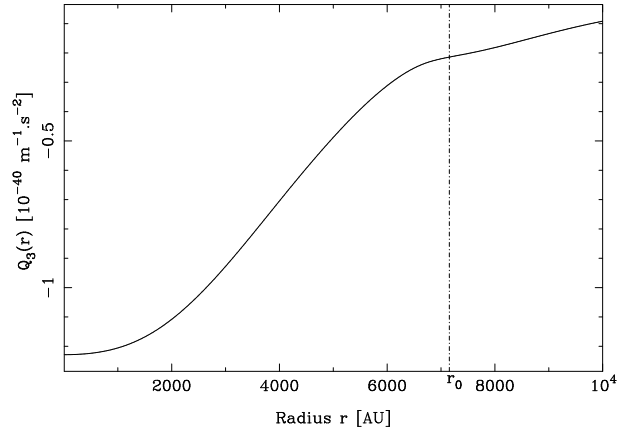
Figure 5. Profiles of dipole Q_1(r) (left) and octupole Q_3(r) (right) in the solar system, with same settings as those of Fig. 4. The MOND transition radius r_0 = \sqrt{GM/a_0} is shown by a dash-dotted line at r \simeq 7100 AU. Numerically we get |Q_1(0)| \sim 9 \times 10^{-14} \text{ m.s}^{-2} \ll a_0 which shows that the dipole is in fact zero.
