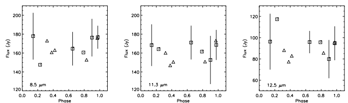
Fig. 6. MIDI (squares) and ISO/SWS (triangles) flux of R Scl as a function of the visual phase in the 8.5 (left), 11.3 (middle), and 12.5 \mu\text{m} (right) spectral band corresponding to the pseudo-continuum , the SiC feature, and the \text{C}_2\text{H}_2 + \text{HCN} feature, respectively.
