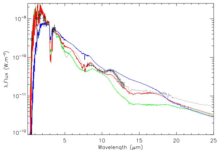
Fig. 12. Synthetic spectra based on the dynamic models at phase 0.98 with piston velocities of 2 (green line), 4 (red line), and 6 \text{km s}^{-1} (blue line), keeping the same parameter values as the ones contained in Table 7. The dotted line is the ISO/SWS spectrum of the star at phase 0.97, whereas the error bars in the N-band correspond to the MIDI fluxes at phase 0.98. Squares and triangles correspond to the photometric measurements of the star (see Table 4).
