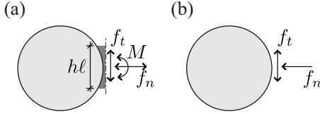
FIG. 1. Schematic representation of the cementation model. (a) Intact cemented bonds support tensile forces, shear forces, and torques. (b) Postrupture contacts are only frictional.
