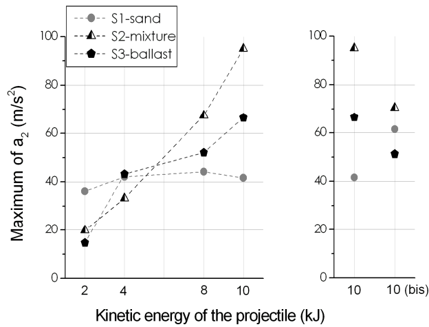
Figure 10. Acceleration at the interface between the front and kernel layers - all the tests
