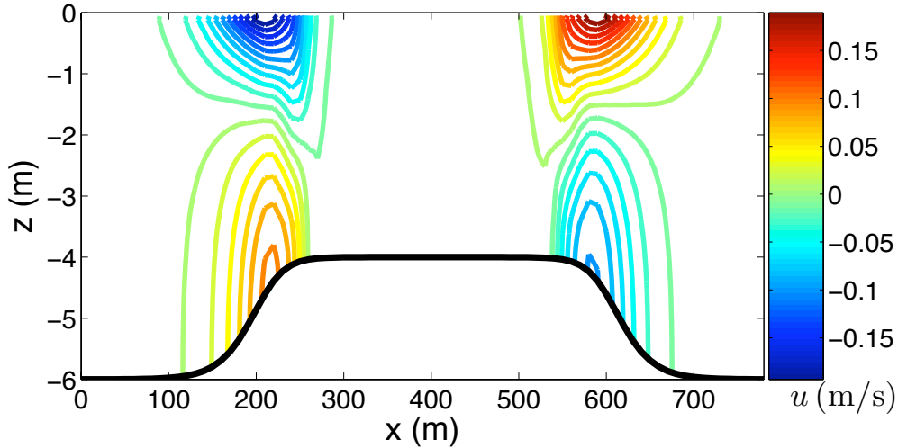
Figure 7: M08 model : Lagrangian velocity U (m/s) of the coupled model after 15 minutes of integration with H_s = 1.02 m, T = 5.24 s, K_z = 2.8 \cdot 10^{-3} \text{ m}^2 \cdot \text{s}^{-1} . The thick black line is the bottom elevation.
