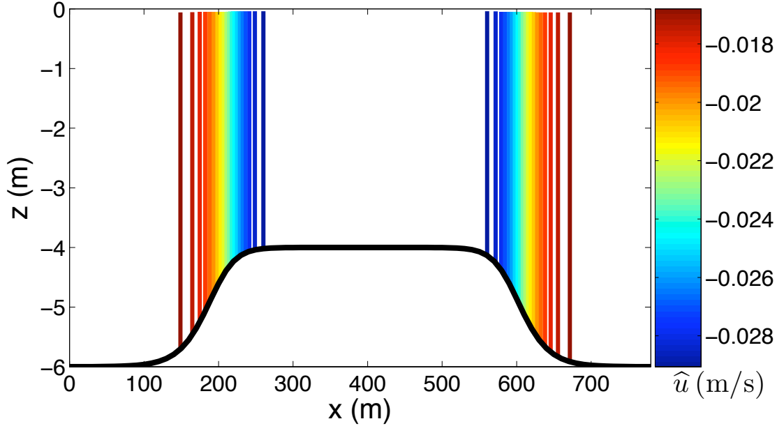
Figure 10: ABR08 model : Quasi-Eulerian velocity \hat{u} (m/s) of the coupled model when a steady state is reached and with H_s = 1.02 m, T = 5.24 s and K_z = 0 \text{ m}^2 \cdot \text{s}^{-1} . The thick black line is the bottom elevation.
