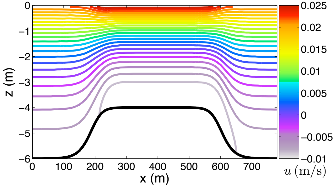
Figure 9: ABR08 model : Lagrangian velocity U (m/s) of the coupled model when a steady state is reached and with H_s = 1.02 m, T = 5.24 s and K_z = 0 m 2 .s -1 . The thick black line is the bottom elevation.
