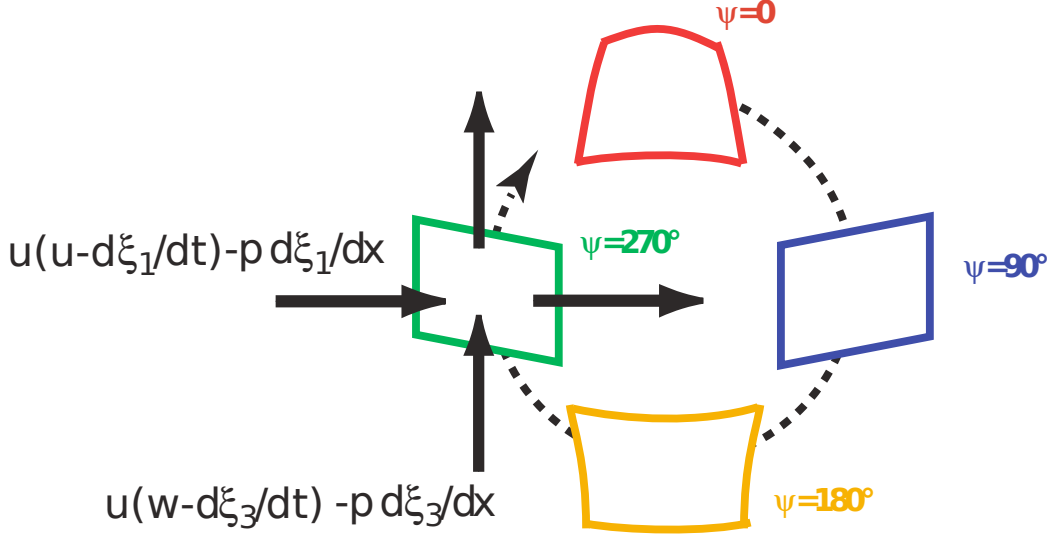
Figure 2: Illustration of the momentum fluxes into a moving control volume defined by the (possibly moving) position vector of the control volume, \Xi(x, y, z, t) = \mathbf{x} + \xi . Here the control volume moves in a circle and is shown for 4 wave phase, \psi = 0^\circ , \psi = 90^\circ , \psi = 180^\circ and \psi = 270^\circ . The fluxes are the sum of advective fluxes through the facets and the pressure acting on the possibly sloping facets. For the advective part the velocity is relative to the moving facet, which leads to terms like -u\partial\xi_3/\partial t .
