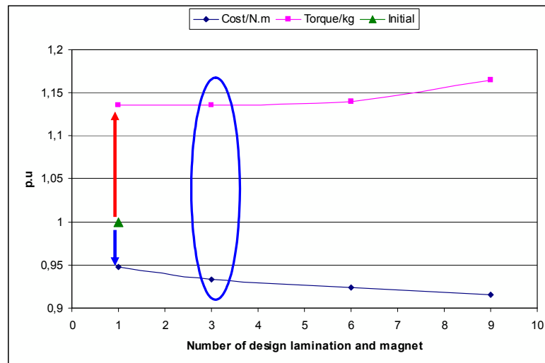
Figure 1. Pareto curves of ranges.
