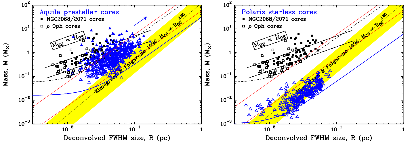
Fig. 4. Mass vs. size diagrams for the starless cores detected with Herschel -SPIRE/PACS in Aquila (left) and Polaris (right) (blue triangles). The masses were derived as explained in Appendix A (see also Könyves et al. 2010) and the sizes were measured at 250\ \mu\text{m} . For reference, the locations of the (sub)mm continuum prestellar cores identified by Motte et al. (1998, 2001) in \rho Oph and NGC2068/2071, respectively, are shown, along with the correlation observed for diffuse CO clumps (shaded band – cf. Elmegreen & Falgarone 1996). The two black solid lines mark the loci of critically self-gravitating isothermal Bonnor-Ebert spheres at T = 7 K and T = 20 K, respectively. The 341 cores classified as prestellar by Könyves et al. (2010), out of a total of 541 starless cores in Aquila, are shown as filled triangles in the left panel. The 302 starless cores of Polaris lie much below the two Bonnor-Ebert lines in the right panel, suggesting they all are unbound. The red solid lines are two lines of constant mean column density at N_{\text{H}_2} = 10^{21}\ \text{cm}^{-2} and N_{\text{H}_2} = 10^{22}\ \text{cm}^{-2} , respectively. The 5\sigma detection threshold at d = 150 pc of existing ground-based (sub)mm (e.g., SCUBA) surveys as a function of size is shown by the dashed curve. (The shape of this curve reflects a constant sensitivity to column density until source size approaches the beam size.) The 5\sigma detection thresholds of our SPIRE 250\ \mu\text{m} observations, given the estimated levels of cirrus noise (cf. Sect. 2) and assumed distances of 260 pc for Aquila and 150 pc for Polaris, are shown by the blue curves. The blue arrow in the left panel indicates how the positions of the Herschel cores (and the blue curve marking the detection threshold) would move in the diagram if a distance of 400 pc were adopted for Aquila instead of 260 pc (see Appendix A).
