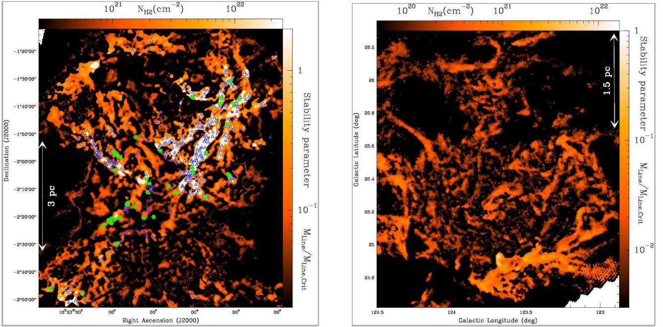
Fig. 1. Column density maps of two subfields in Aquila (left) and Polaris (right) derived from our SPIRE/PACS data. The contrast of the filaments with respect to the non-filamentary background has been enhanced using a curvelet transform as described in Appendix A. Given the typical width \sim 10000 AU of the filaments, these column density maps are equivalent to maps of the mass per unit length along the filaments . The color scale shown on the right of each panel is given in approximate units of the critical line mass of Inutsuka & Miyama (1997) as discussed in Sect. 4. The areas where the filaments have a mass per unit length larger than half the critical value and are thus likely gravitationally unstable have been highlighted in white. The maximum line mass observed in the Polaris region is only \sim 0.45 \times the critical value, suggesting that the Polaris filaments are stable and unable to form stars at the present time. The candidate Class 0 protostars and bound prestellar cores identified in Aquila by Bontemps et al. (2010) and Könyves et al. (2010) are shown as green stars and blue triangles, respectively. Note the good correspondence between the spatial distribution of the bound cores/protostars and the regions where the filaments are unstable to gravitational collapse.
