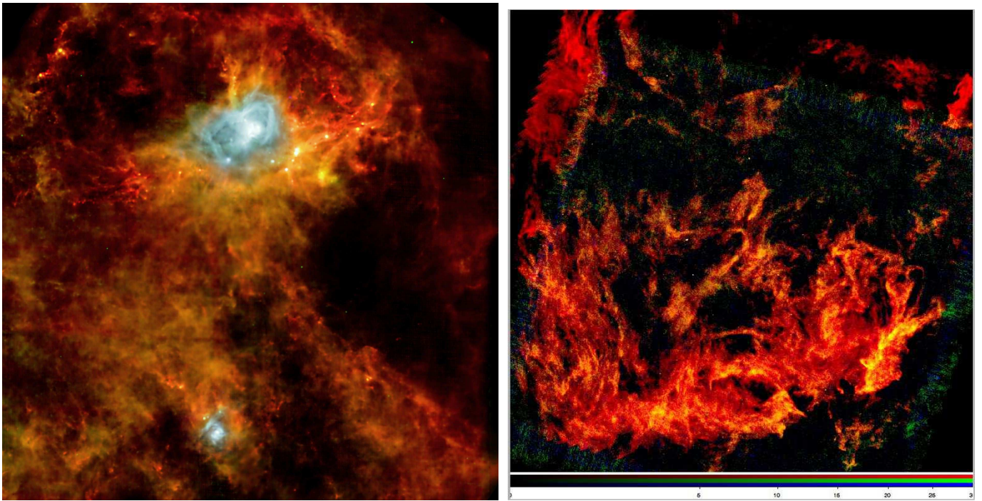
Fig. 3. Composite 3-color images of the \sim 11 \text{ deg}^2 Aquila field ( left ) and the \sim 8 \text{ deg}^2 Polaris field ( right ) produced from our PACS/SPIRE parallel-mode images at 70, 160, and 500 \mu\text{m} . The color coding of the Aquila image is such that Red = SPIRE 500 \mu\text{m} , Green = PACS 160 \mu\text{m} , Blue = PACS 70 \mu\text{m} . For the Polaris image, Red = combination of the three SPIRE bands, Green = PACS 160 \mu\text{m} , Blue = PACS 70 \mu\text{m} . The Aquila composite image was also the first release of “OSHI”, ESA’s Online Showcase of Herschel Images (cf. http://oshi.esa.int and http://www.esa.int/SPECIALS/Herschel/SEMT0T9K73G_0.html ).
