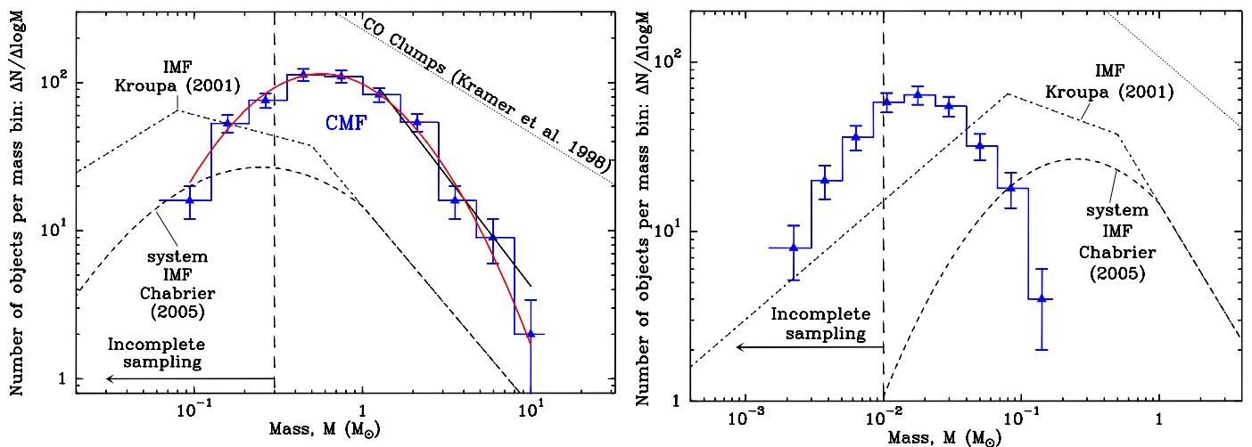
Fig. 2. Core mass functions (blue histograms with error bars) derived from our SPIRE/PACS observations of the Aquila (left) and Polaris (right) regions, which reveal of total of 541 candidate prestellar cores and 302 starless cores, respectively. A lognormal fit (red curve) and a power-law fit (black solid line) to the high-mass end of the Aquila CMF are superimposed in the left panel. The power-law fit has a slope of -1.5 \pm 0.2 (compared to a Salpeter slope of -1.35 in this dN/d\log M format), while the lognormal fit peaks at \sim 0.6 M_{\odot} and has a standard deviation of \sim 0.43 in \log_{10} M . The IMF of single stars (corrected for binaries – e.g., Kroupa 2001), the IMF of multiple systems (e.g., Chabrier 2005), and the typical mass spectrum of CO clumps (e.g., Kramer et al. 1998) are also shown for comparison. Note the remarkable similarity between the Aquila CMF and the stellar IMF, suggesting a \sim one-to-one correspondence between core mass and star/system mass with M_{\star, \text{sys}} = \epsilon M_{\text{core}} and \epsilon \approx 0.4 in Aquila.
