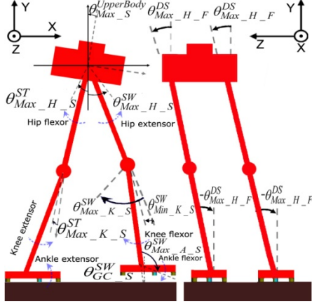
Fig. 3. Extreme angles characterizing ROBIAN Locomotion
