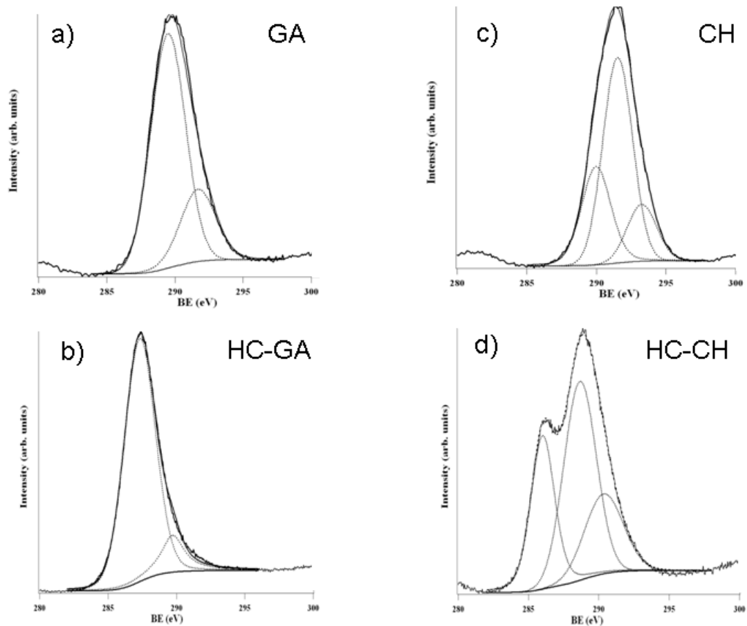
Fig. S 4 – C1s signals of the pure and hydrothermally treated glucosamine (GA) and chitosan (CH) samples. The values in the abscissa are not corrected for the charging effects. Refer to discussion in the text or to
