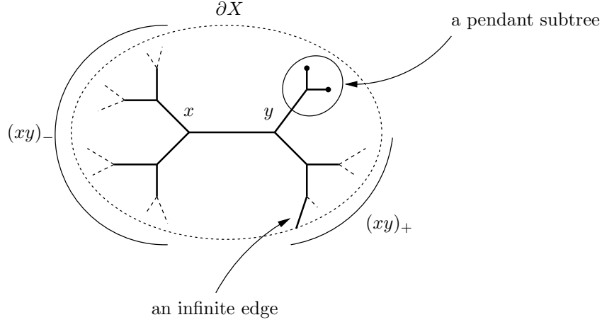
FIGURE 5. The edge (xy) is positive if \nu_+((xy)_+) > \nu_-((xy)_+) since this means that some mass has to move through (xy) (in this direction). The edges of the pendant subtree (finite complement of a vertex) are all neutral.
