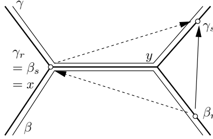
FIGURE 6. Antagonist pairs of geodesics contradict the cyclical monotonicity: the transport plan corresponding to the solid arrow is cheaper than the one corresponding to the dashed arrows.
