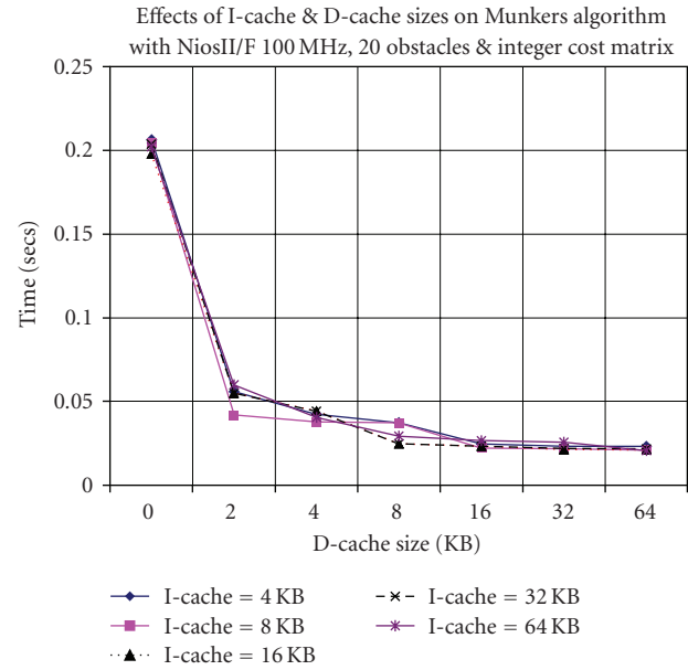
FIGURE 21: Cache Behavior for Munkres Algorithm with Integer Cost Matrix.
