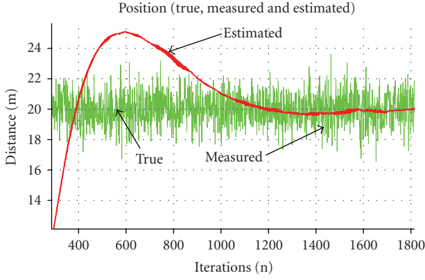
FIGURE 5: Estimated target position.
