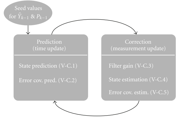
FIGURE 4: The Kalman filter.
