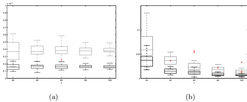
Figure 4: Boxplot of \frac{1}{J}\|\hat{\boldsymbol{\theta}}^\lambda - \boldsymbol{\theta}_{\Theta_0}^*\|^2 (a) and \|\hat{f}^\lambda - f_{\Theta_0}^*\|_{L^2}^2 (b) over M = 20 repetitions from a SIM model of shifted curves. Boxplot in gray correspond to n = 512 , and in black to n = 1024 .
