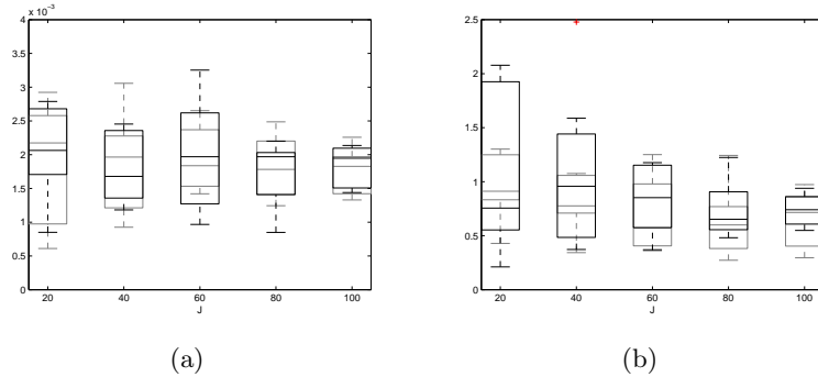
Figure 6: Boxplot of \frac{1}{J} \|\hat{\theta}^\lambda - \theta_{\Theta_0}^*\|^2 (a) and \frac{1}{J} \|\hat{f}^\lambda - f_{\Theta_0}^*\|^2 (b) in model (3.1) with a non-stationary error term Z . Boxplot in grey correspond to n = 512 , and in black to n = 1024 .
