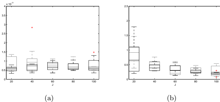
Figure 5: Boxplot of \frac{1}{J} \|\hat{\theta}^\lambda - \theta_{\Theta_0}^*\|^2 (a) and \frac{1}{J} \|\hat{f}^\lambda - f_{\Theta_0}^*\|^2 (b) in model (3.1) with a stationary error term Z . Boxplot in gray correspond to n = 512 , and in black to n = 1024 .
