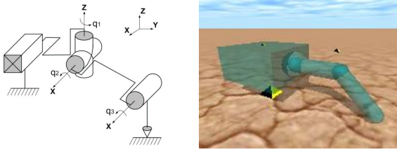
Figure 2: Morphology of the single-legged robot. Left: Kinematic model. Right: Simulation view.
