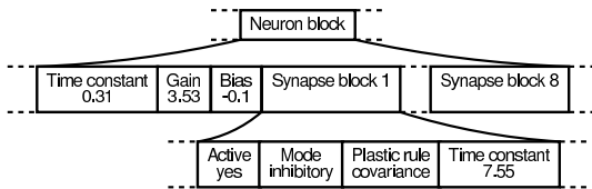
Figure 4: Structure of the neuron genotype.
