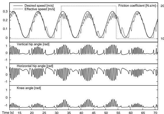
Figure 7: Time-plots of V_{des} , \widetilde{V}_{eff} , k_{fr} and joint commands for a CCNS controller. The robot is perturbed from t = 32 sec during about 22 sec. Robot strides cause light oscillations of \widetilde{V}_{eff} (attenuated by the low-pass filter).
