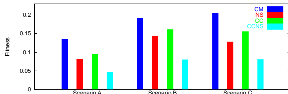
Figure 6: Average fitness of the best controllers (one from each evolution run), according to a scenario and a neural model. Fitness are evaluated during a simulation of 100 sec.
