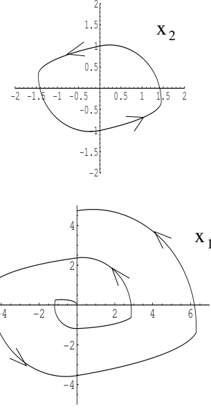
Fig. 1. Example 3.2: Trajectory of a polynomially unstable switched system
