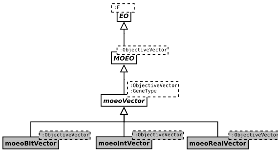
Fig. 5.2. UML diagram for the representation of a solution
