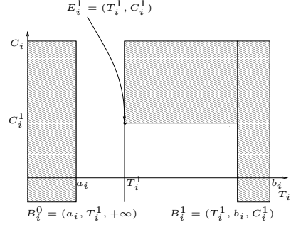
Figure 3: Label expansion
