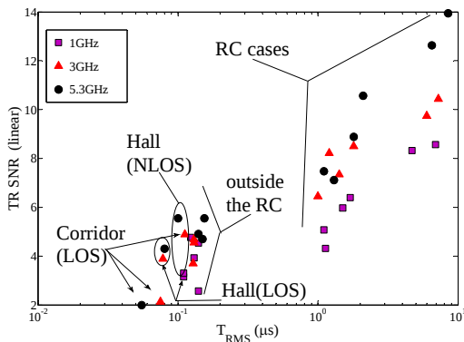
Fig. 6. The TR SNR versus the delay spread T_{\text{RMS}} computed in the different configurations.
