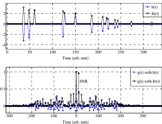
Fig. 1. (a) Example of a channel response h(t) with fifteen \alpha_i and its absolute value |h(t)| . (b) Respective computed normalized autocorrelation function. The influence of the sign repartition of the \alpha_i has a direct influence on the side-peaks amplitudes.
