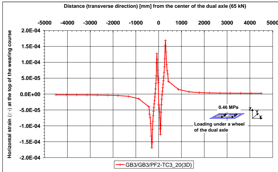
Figure 5: Transverse strain at the top of the surface layer
