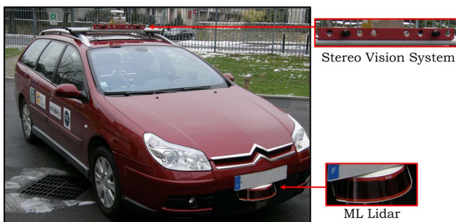
Figure 3. The experimental vehicle with the stereo vision system and the IBEO Alasca XT
