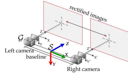
Figure 4. Stereo Vision System Model
