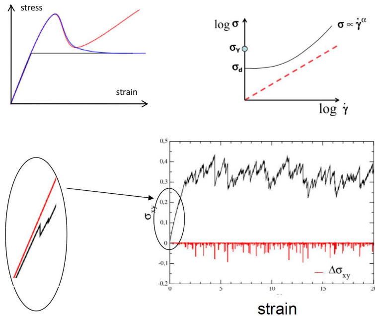
Fig. 0.1 Top left: schematic illustration of a stress strain curve for the plastic deformation of a solid material. The three curves correspond respectively to ideal elastoplastic behavior, a metallic and a polymeric system at finite strain rate. The strain hardening part at large strain is specific of polymer systems. Top right: schematic illustration of a flow curve for a soft material; the dotted line is the Newtonian fluid case, the low strain rate limit of the full curve corresponds to the yield stress. Bottom: actual response of a simulated strained glass at low temperature. Note the large stress fluctuations, that are associated with the finite size of the sample. The stress variations are also shown. The zoom on the elastic part at low strain shows that small plastic events are also observed in this part. Adapted from (Tanguy et al. , 2006b)
