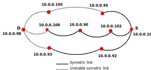
Figure 20: Quality of links in scenario 2: OLSR and MP-OLSR with 3 paths
