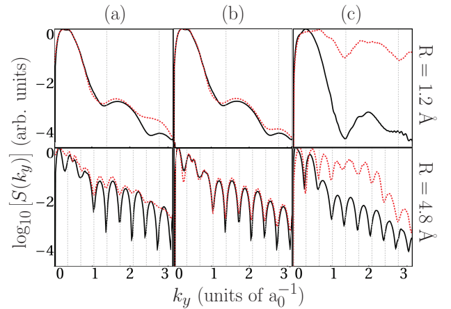
FIG. 3. (Color online) Averaged normalized electron diffraction patterns S(k_y) resulting from ionizing the HOMO of \text{CO}_2 under the same field conditions as in Fig. 1 for R = 1.2 \text{ \AA} (first row) and R = 4.8 \text{ \AA} (second row). The solid black lines correspond to a perfect alignment at fixed internuclear distance for a single optical cycle pulse. The red dashed lines correspond to, column (a), an imperfect alignment, column (b), a distribution of R and, column (c), a 10 fs FWHM sine-square pulse.
