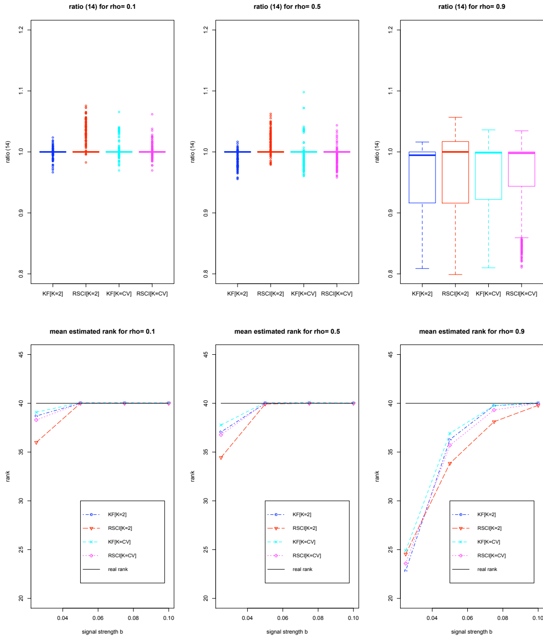
FIGURE 3. Experiment 1. Left to right : \rho = 0.1, 0.5, 0.9 . Top : boxplots of the ratio (14) for \text{KF}[K = 2] , \text{RSCI}[K = 2] , \text{KF}[K = CV] and \text{RSCI}[K = CV] . Bottom : mean estimated rank \mathbb{E}[\hat{r}] for each estimator and each value of b .
