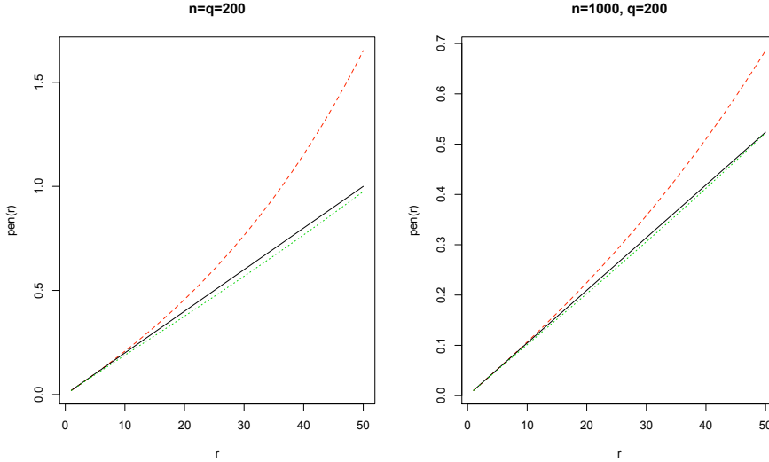
FIGURE 2. In dotted green \text{pen}(r) = -\log(1 - \mathcal{S}_{q \times n}(r)^2/(nq - 1)) , in solid black \text{pen}(r) = r(\sqrt{n} + \sqrt{q})^2/(nq) , in dashed red \text{pen}'(r)/(nq) = \mathcal{S}_{q \times n}(r)^2/(nq - 1 - \mathcal{S}_{q \times n}(r)^2) . Left : q = n = 200 . Right : q = 200 and n = 1000 .
