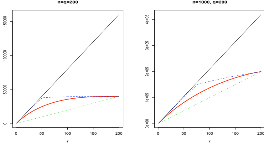
FIGURE 1. In bold red r \rightarrow \mathcal{S}_{q \times n}(r)^2 , in solid black r \rightarrow r(\sqrt{n} + \sqrt{q})^2 , in dashed blue the upper-bound of Lemma 1, in dotted green the lower bound. Left: q = n = 200 . Right: q = 200 and n = 1000 .
