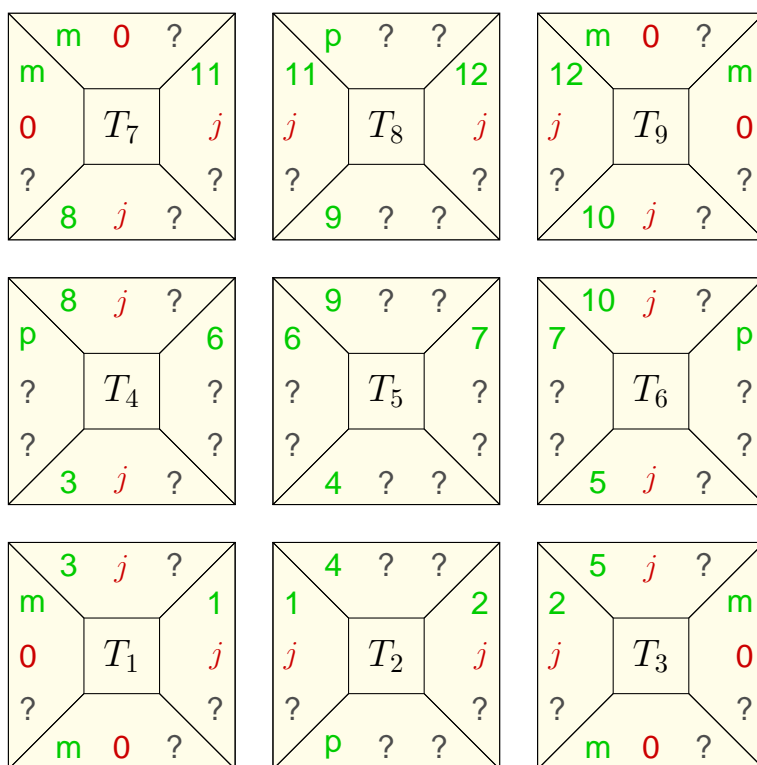
Figure 13: after step 2: parent-indices are fixed outside network
