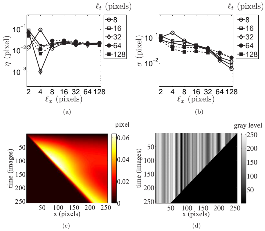
Figure 4: Systematic error (a) and standard uncertainty (b) as functions of the element size for the measured displacement field. Difference between the prescribed and measured displacement fields for 128 \times 128 -pixel elements (c). Reconstruction of the corrected map g by using the measured displacement field for 8 \times 8 -pixel elements (d).
