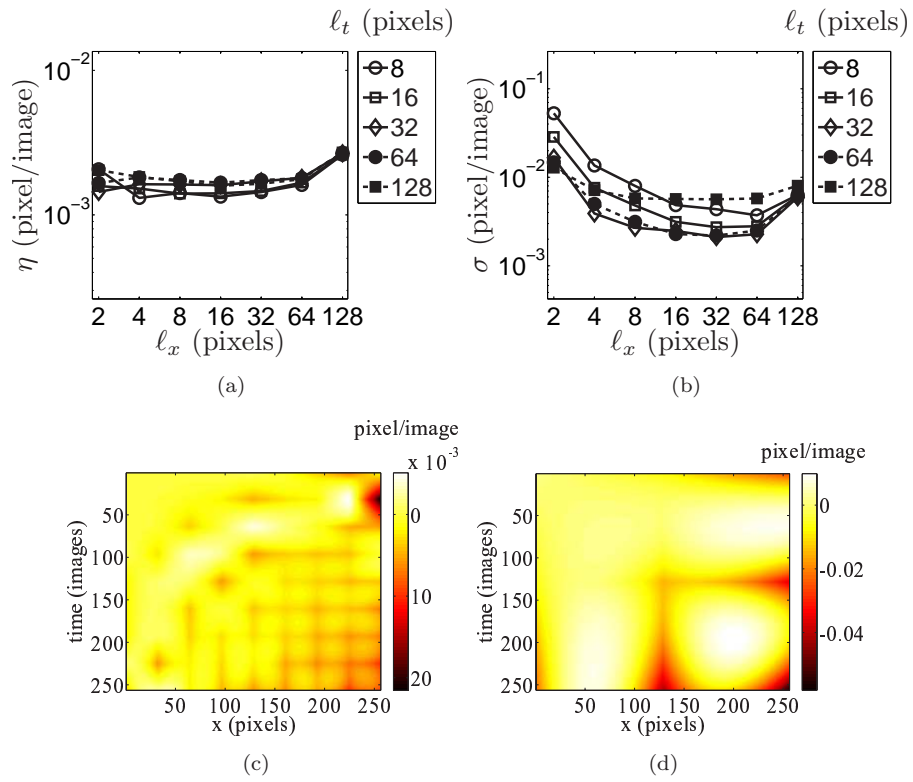
Figure 7: Systematic error (a) and standard uncertainty (b) as functions of the element size for the measured velocity field when a parabolic velocity is prescribed. Difference between the prescribed and measured velocity fields for 32 \times 32 -pixel elements (c), and 128 \times 128 -pixel elements (d).
