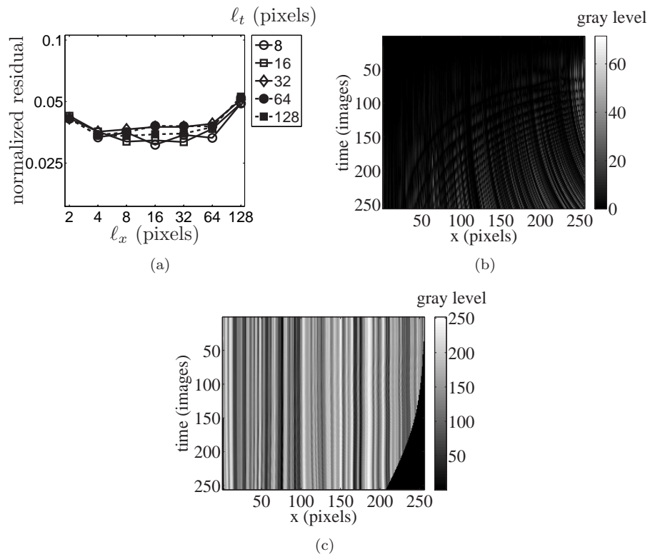
Figure 8: Normalized mean gray level residual as a function of element size for a parabolic prescribed velocity (a). Residual map between the measured (with 32 \times 32 -pixel elements) and the prescribed trajectories (b). Corrected map with the measured displacement field for a 32 \times 32 pixel element (c).
