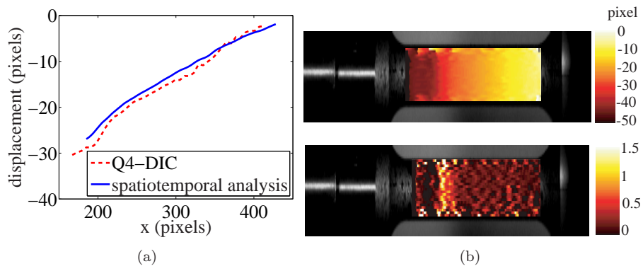
Figure 13: Comparison between the displacement field given by the spatiotemporal approach and a Q4-DIC technique (a), the element size is equal to 6 \times 6 pixels for Q4-DIC and 4 \times 12 pixels for the spatiotemporal approach. Displacement and engineering strain maps computed with the proposed approach for image no. 175 (just before failure) (b).
