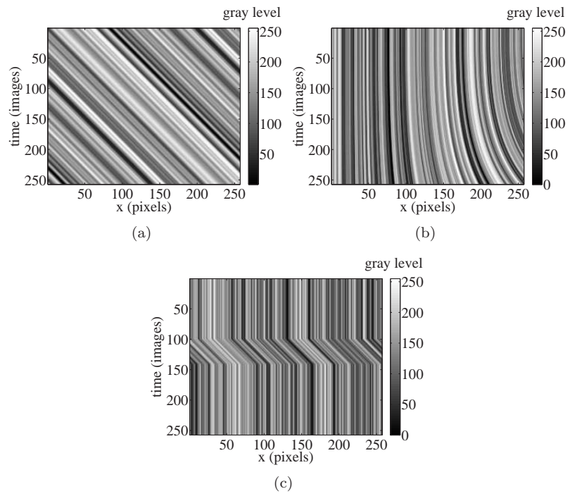
Figure 2: Spatiotemporal map corresponding to a constant velocity (a), a parabolic velocity field (b) and a discontinuous velocity field (c).
