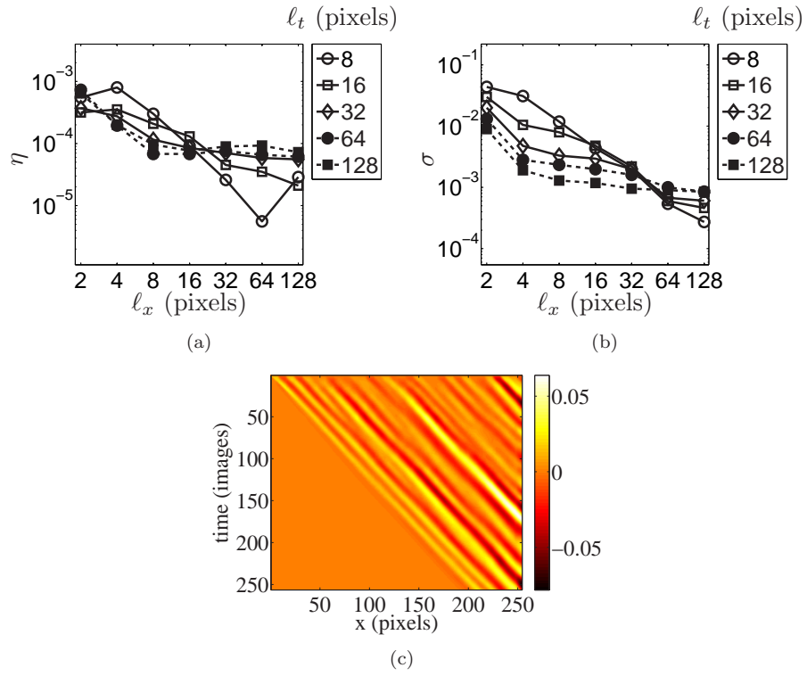
Figure 6: Systematic error (a) and standard uncertainty (b) as functions of the element size for the strain field. Difference between the prescribed and measured strain fields for an element of size 8 \times 8 pixels (c).
