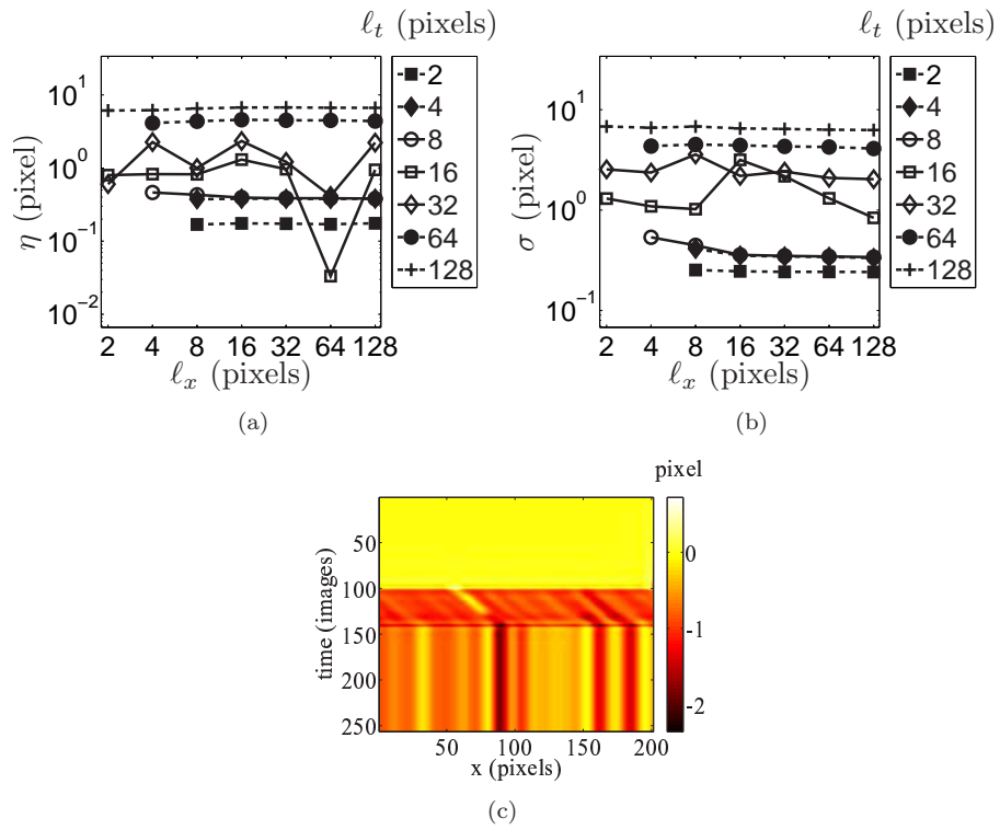
Figure 10: Systematic error (a) and standard uncertainty (b) as functions of the element size for the displacement field when a discontinuous velocity field is prescribed. Difference between the prescribed and measured displacement fields for 8 \times 8 -pixel elements (c).
