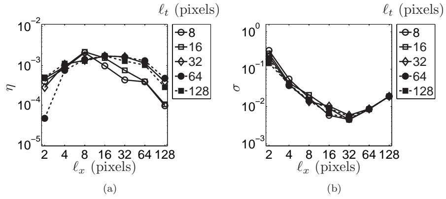
Figure 9: Systematic error (a) and standard uncertainty (b) as functions of the element size, for the measured strain field when a parabolic velocity field is prescribed.
