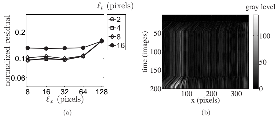
Figure 14: Normalized mean gray level residual as function of element size for the real application (a). Difference between the real and reconstructed spatiotemporal maps (b). The latter is reconstructed with the measured velocities ( 4 \times 20 -pixel elements).
