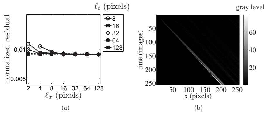
Figure 5: Normalized mean gray level residual as a function of the element size for a constant prescribed velocity (a). Residual map between the measured (with 8 \times 8 -pixel elements) and prescribed trajectories (b).
