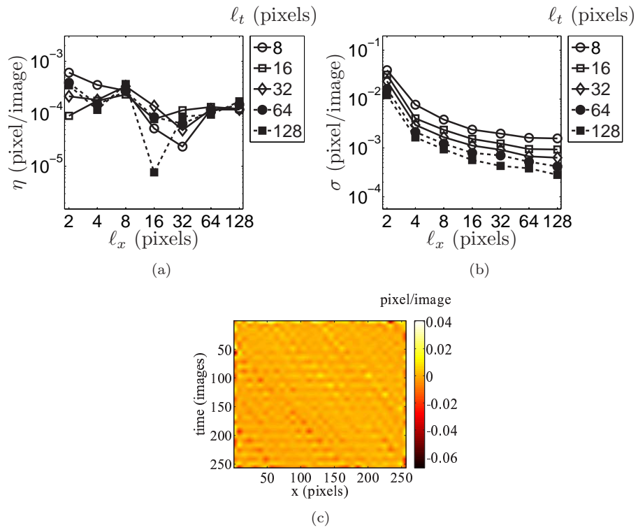
Figure 3: Systematic error (a) and standard uncertainty (b) as functions of the element sizes for the measured velocity field. Difference between the prescribed and measured velocity fields for 8 \times 8 -pixel elements (c).
