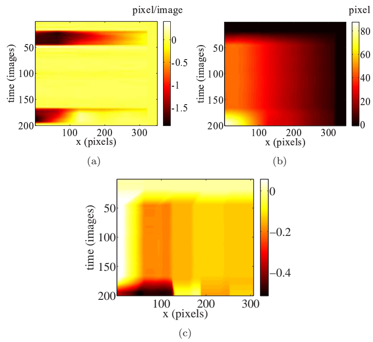
Figure 12: Velocity (a), displacement (b) and engineering strain (c) maps for the studied test.
