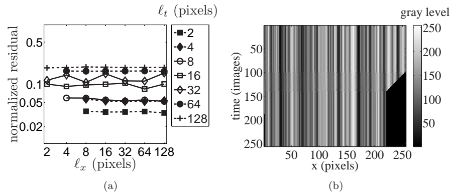
Figure 11: Normalized mean gray level residual as a function of the element size for a discontinuous prescribed velocity (a). Corrected map for 8 \times 8 -pixel elements (b).
