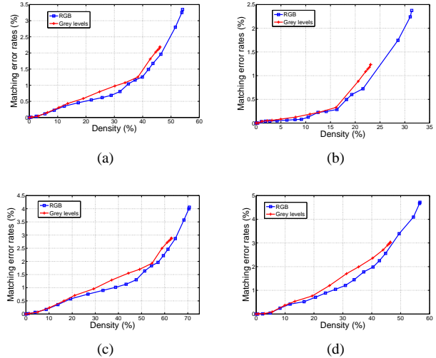
Fig. 6. Matching error rates versus density rates based on the disparity maps computed with grey level images and RGB images in: (a) non-occluded areas ( B_{\overline{O}} ), (b) non-textured areas ( B_{\overline{T}} ), (c) textured areas ( B_{\mathcal{T}} ), and (d) discontinuities ( B_{\mathcal{D}} )
