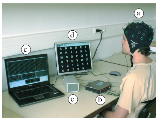
(1) hardware setup
