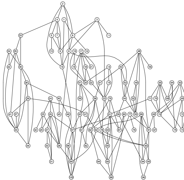
FIG. 9. Synthetic data: Random graph used in the evaluation of the pruning procedure.
