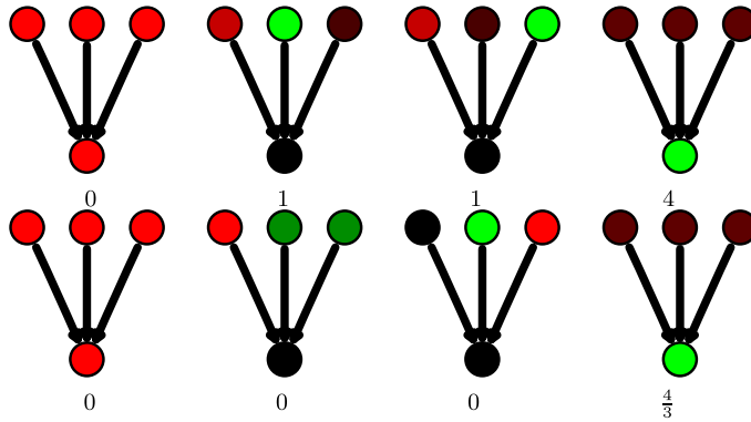
FIG. 3. Eigenvectors of the signed Laplacian \mathcal{L}_{\text{sign}} (top) and of M_G (bottom) for the simple directed four-node graph of example (2.4). The corresponding eigenvalues are 0, 1, 1, 4 and 0, 0, 0, \frac{4}{3} , respectively. Nodes are colored according to the value of the eigenvector, where green corresponds to high positive values, red to high negative values, and black to 0.
