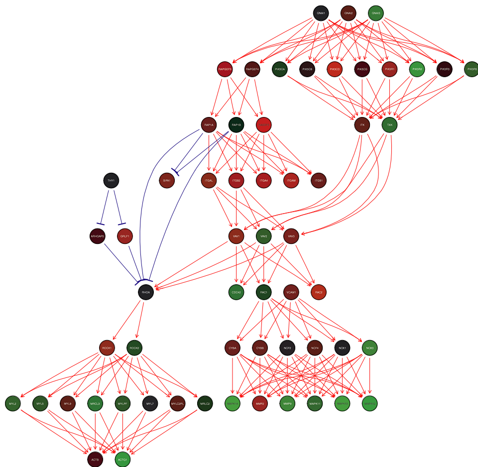
FIG. 12. Breast cancer data set: KEGG leukocyte transendothelial migration pathway. Scaled difference in sample mean expression measures between tamoxifen-resistant and sensitive patients, for genes in one component of the KEGG leukocyte transendothelial migration pathway. Nodes are colored according to the value of the difference in means, with green corresponding to high positive values, red to high negative values, and black to 0. Red arrows denote activation, blue arrows inhibition.
