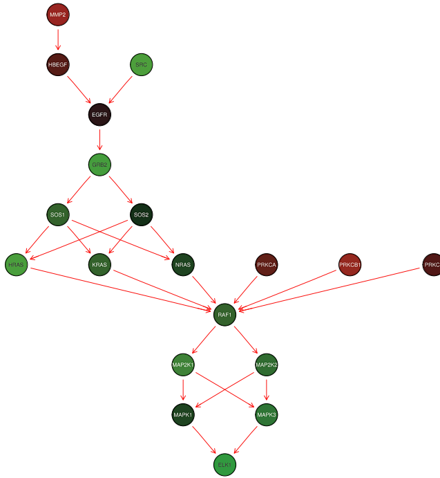
FIG. 11. Breast cancer data set: KEGG GnRH signaling pathway. Scaled difference in sample mean expression measures between tamoxifen-resistant and sensitive patients, for genes in one component of the KEGG GnRH signaling pathway. Nodes are colored according to the value of the difference in means, with green corresponding to high positive values, red to high negative values, and black to 0. Red arrows denote activation, blue arrows inhibition.
