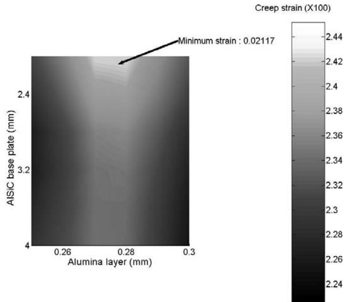
Figure 5: creep strain following the AISiC and the alumina thicknesses.
