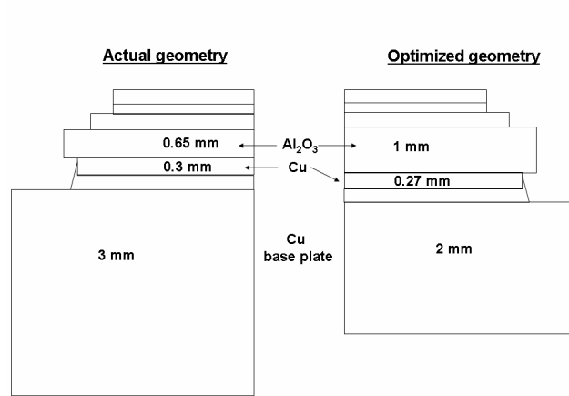
Figure 6: Actual and optimized geometries
