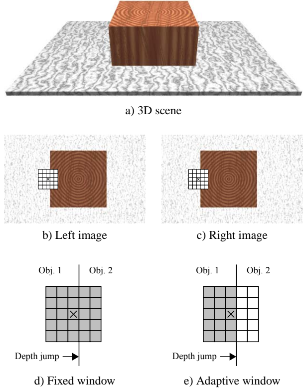
Fig. 1. Fixed versus adaptive window
