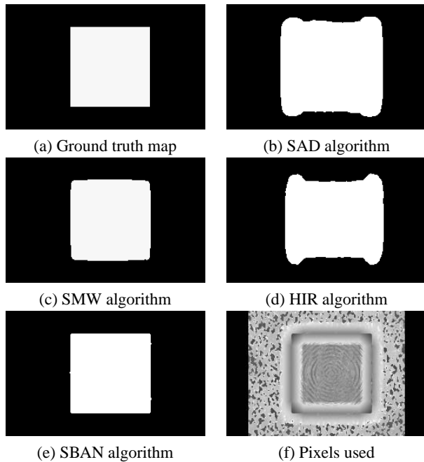
Fig. 3. Results for the synthetic pair (window size 31 \times 31 )
