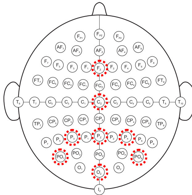
Fig. 2. The electrode montage used in the current study [15]. The 8 electrodes selected for analysis are indicated by the dotted circles.
