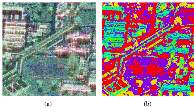
Fig. 1. Classification results for the X-band RAMSES data over the Toulouse test-site ( 700 \times 700 pixels) : (a) Colored composition of the target vector [k]_1 - [k]_3 - [k]_2 . (b) Classification using the Wishart criterion.
