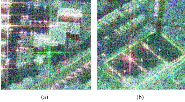
Fig. 2. Toulouse, RAMSES PolSAR data, X-band ( 150 \times 150 pixels). Colored composition in the Pauli basis of the target vector [k]_1 - [k]_3 - [k]_2 . Images containing a dihedral (a) and a narrow diplane (b).
