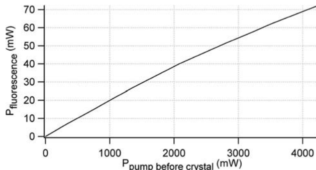
Fig. 6. Output fluorescent power sent into the FF-OCT setup versus incident pump power.
