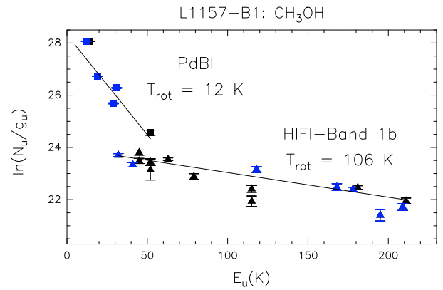
Fig. 4. Rotation diagrams for the \text{CH}_3\text{OH} transitions measured with HIFI (triangles) and from ground (PdBI; squares). Black and blue points are for A- and E-form, respectively. The parameters N_u , g_u , and E_u are, respectively, the column density, the degeneracy and the energy (with respect to the ground state of each symmetry) of the upper level. The derived values of the rotational temperature are reported: (i) 106 K, for the HIFI lines covering the E_u = 32-211 \text{ K} excitation range and (ii) 12 K (as Bachiller et al. 1995), for the PdBI lines, at lower excitation.
