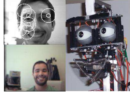
Fig. 11. Joy expressions on unknown faces and at different distances are successfully imitated by the robot head.
