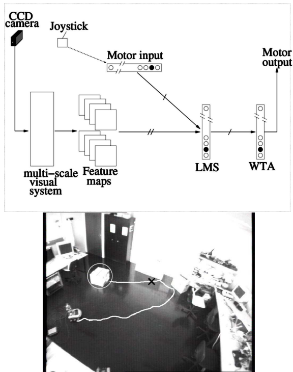
Fig. 7. top: The sensori-motor architecture. bottom: Trajectory of a robot performing an object reaching task. The object enters the robots visual field only at the black cross position.
