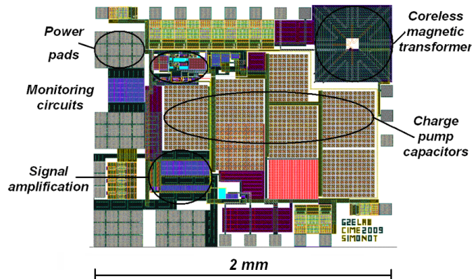
Fig. 4. Layout of the driver/control die with its main functional regions and their necessary electrical interconnections.
