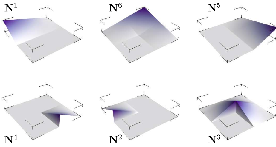
Figure 39: Shape functions associated to the composite element e_{123} .
