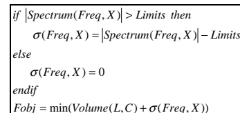
Figure 4: objective function
