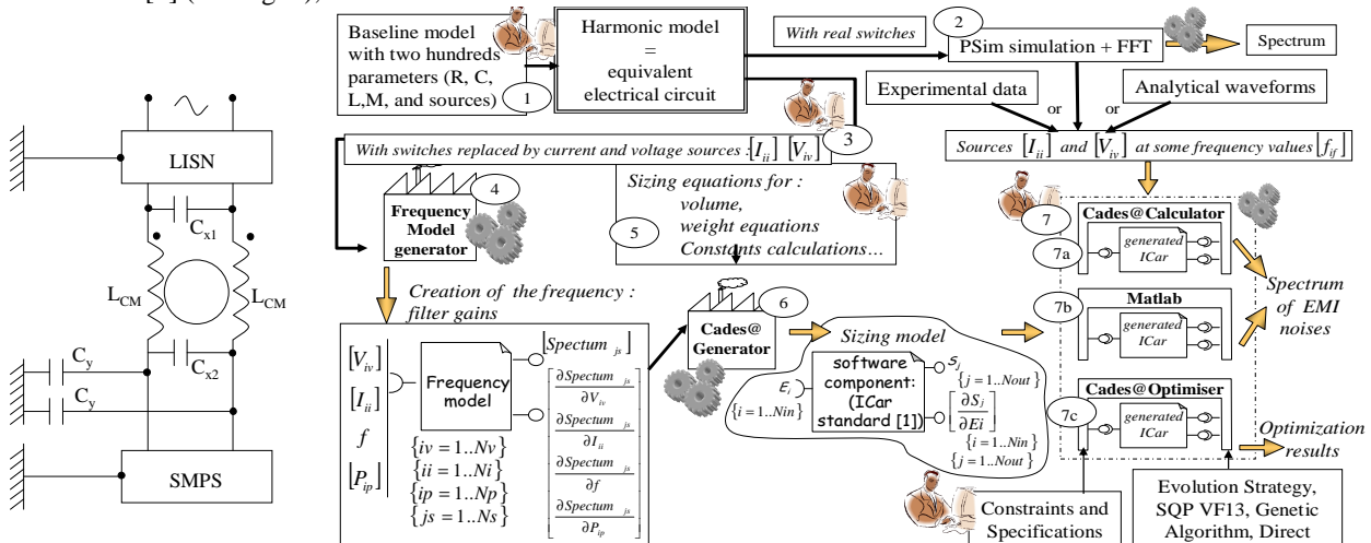
Figure 1: EMI Filter
