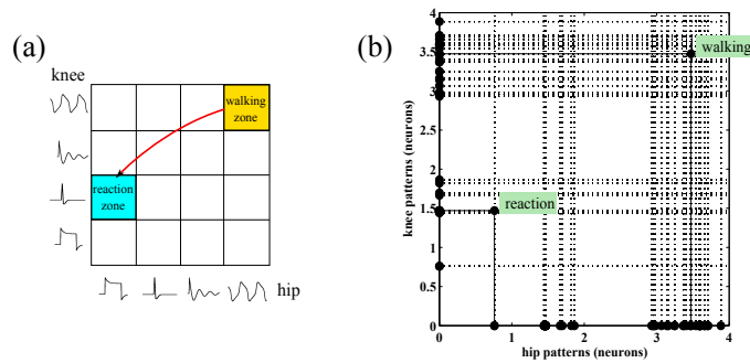
Fig. 7. The space of patterns is for hip and knee joints, with an example of switching against perturbation. (a) Patterns switch from walking by oscillatory patterns to quiescent pattern for knee and plateau for hip. (b) Neurons switch from walking zone to other neurons that represent quiescent pattern for knee and plateau for hip. Each neuron represents one pattern.
