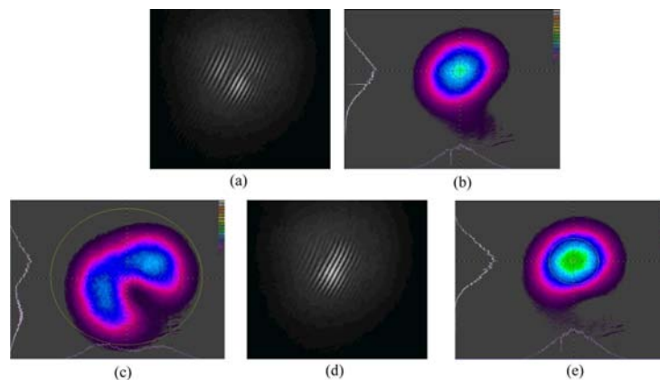
Fig. 7. Application of a pressure to the fiber in the pulsed regime, frame excerpts from Media 2 . (a) Recorded hologram on CCD 1 without pressure. (b) Corresponding output beam on CCD 2. (c) Output beam on CCD 2 with a pressure applied. (d) New recorded hologram after the application of the pressure. (e) Corresponding output beam on CCD 2.
