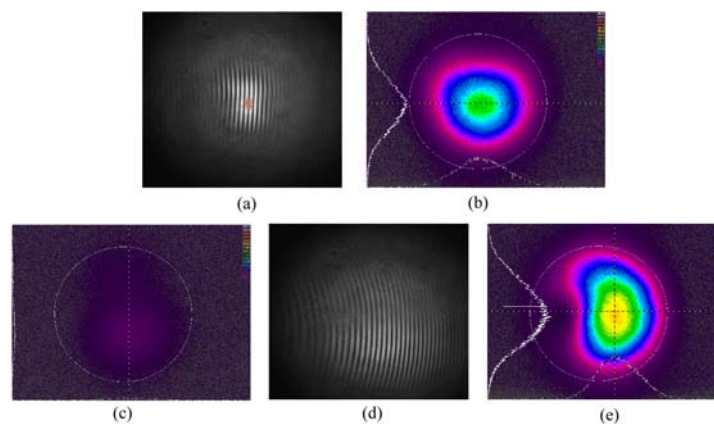
Fig. 4. Compensation of the phase error introduced by a 500 mm focal tilted lens. (a) Recorded hologram on CCD 1 without lens. (b) Corresponding output beam on CCD 2. (c) Output beam on CCD 2 after the insertion of the lens without changing the hologram. (d) New recorded hologram after the insertion of the lens. (e) Corresponding output beam on CCD 2.
