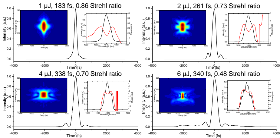
Fig. 2. FROG retrieved pulses at the YDFA output after compression for energies from 1 \mu\text{J} to 6 \mu\text{J} .
