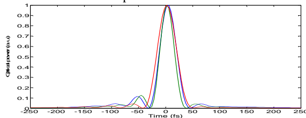
Fig. 4. Temporal profiles of the compressed pulses obtained by numerical simulations of the nonlinear compression in the 5 cm long rod-type fiber for initial chirp of: +15000 \text{ fs}^2 (green line), 0 \text{ fs}^2 (blue line), -15000 \text{ fs}^2 (red line).
