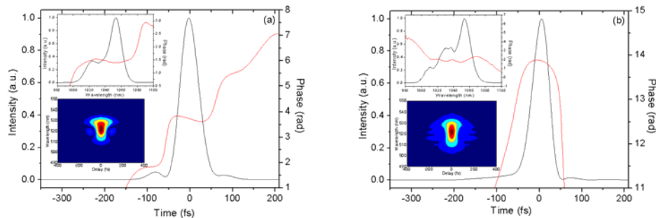
Fig. 3. FROG retrieved temporal and spectral (inset) intensities (black) and phase (red), at 2 \mu\text{J} (left) and 4 \mu\text{J} (right) input energies.
